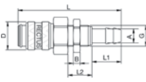
Panel Mount Hose Barb Coupler
