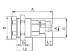
Front Panel Install. Plastic Hose Connection Coupler
