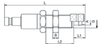
Panel Mount Plastic Hose Connect. Plug
