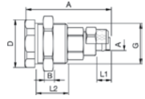
Front Panel Install. Plastic Hose Connection Coupler
