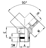
Sprint ® Female-Female-Male "Y"
