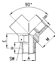
Female-Female-Female "Y"
