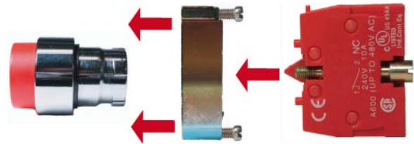
Metal Chrome Bezel Steel Block Holder Included with operators Bolt-On Contact Block
