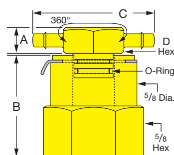
1/8 NPT Female Thread
