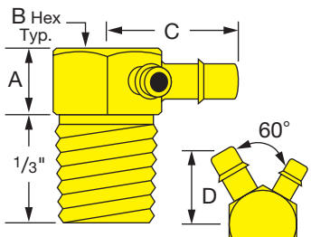
Top View: Right-hand Reducing VT's have the (smaller) Reducing Branch on the right.
