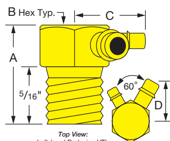
Top View: Left-hand Reducing VT's have the (smaller) Reducing Branch on the left.
