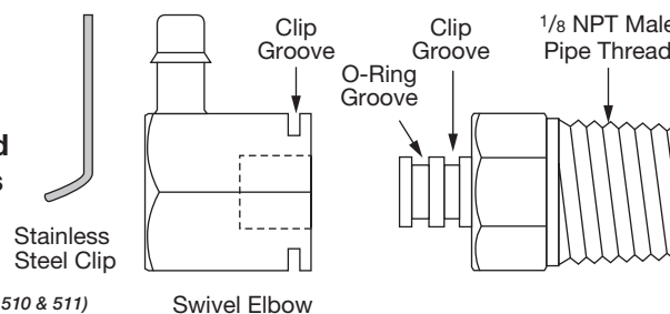
Swivel Elbow
