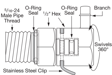
Stainless Steel Clip
