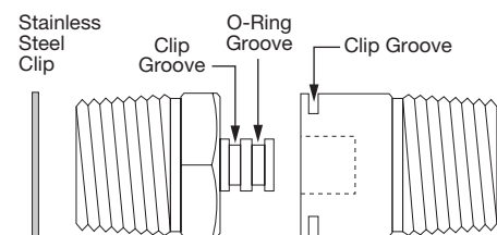
Unassembled Components
