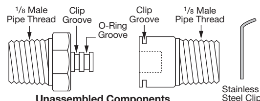
Unassembled Components
