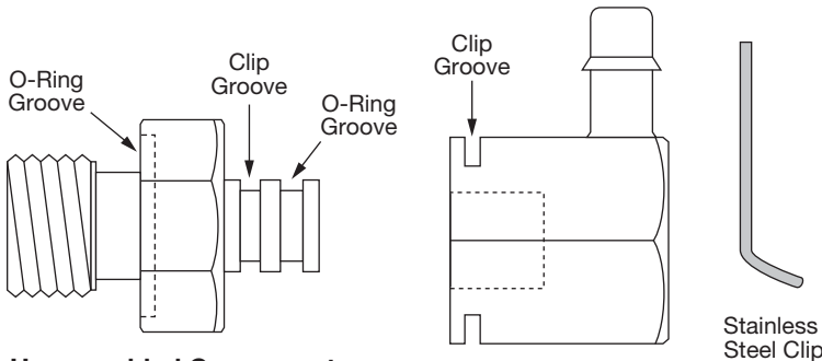
Unassembled Components
