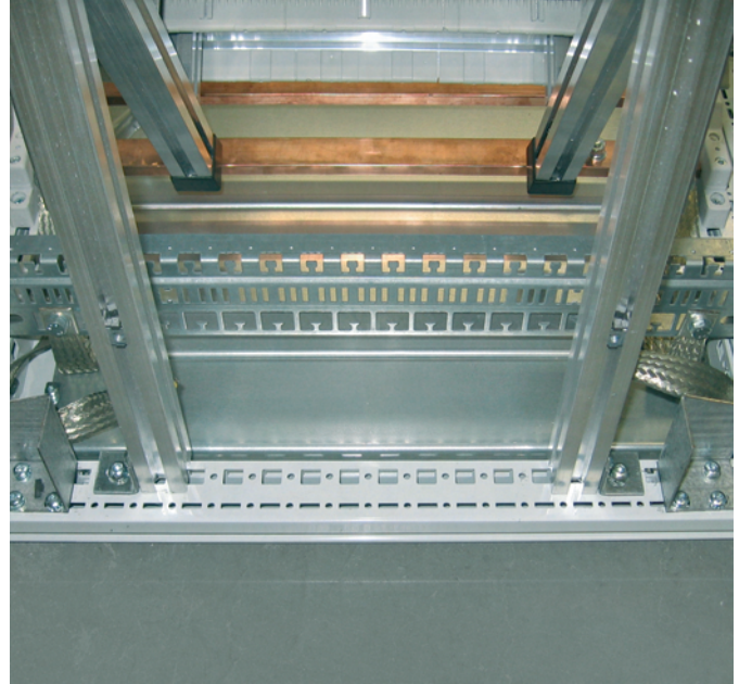
Installation situation in the TS8 cabinet (make Rittal) - fastening of the LSC-Distance frame on mounting brackets
