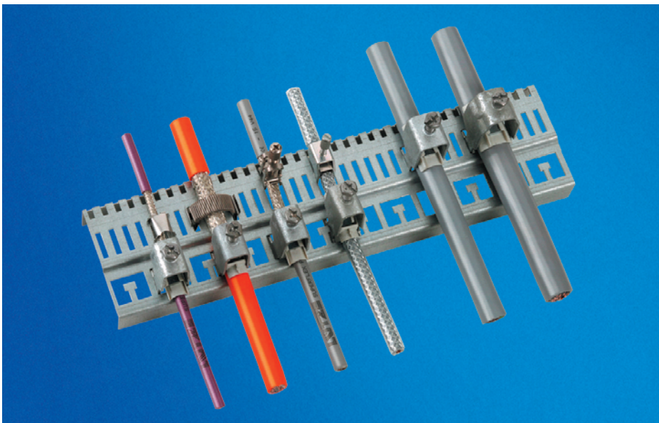
The new generation of EMC rails: For all kinds of shield brackets.
