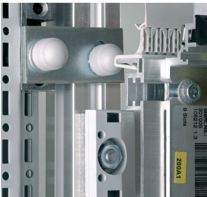
Installation situation, LSC-BRACKET frame
