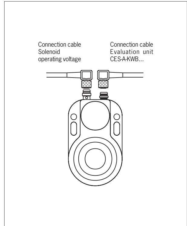
Cable outlet, angled plug connector
