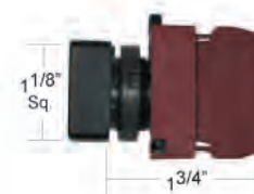
Side view of Square Operator with single contact block.
