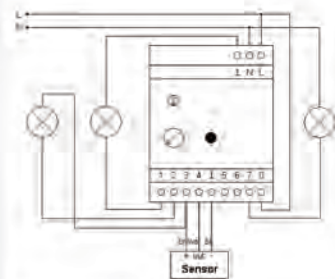
Wiring Example
