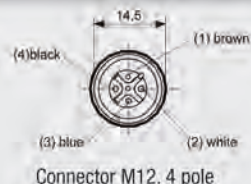
Connector M12, 4 pole
