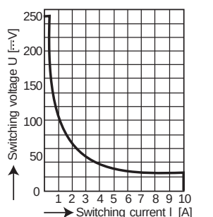
Maximum switching power curve
