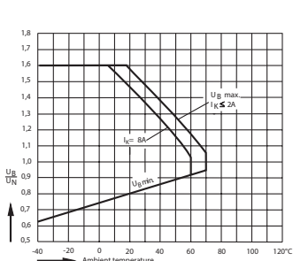
Relay operation voltage vs. ambient temperature
