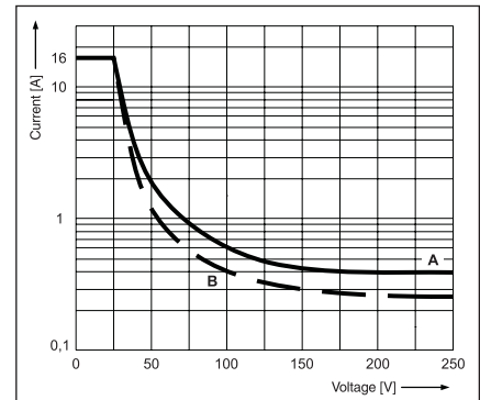
Max. DC breaking capacity A - resistive load DC1 Fig. 3 B - inductive load L/R = 40 ms
