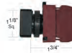
Side view of Square Operator with single contact block.
